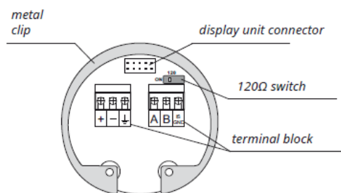
Inside view of screw terminals of the level meter with Modbus EMKOTDR-60_--_-M
