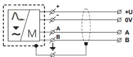
Wiring diagram of the level meter with Modbus EMKOTDR-60_--_-M
