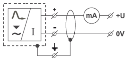
Wiring diagram of the level meter with current output EMKOTDR-60_--_-I
