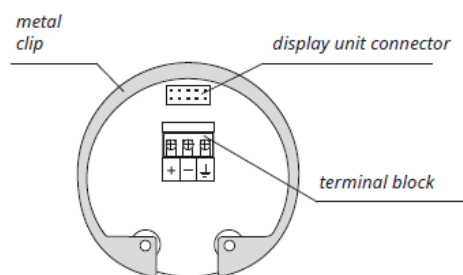
Inside view of screw terminals of the level meter with current output EMKOTDR-60_--_-I
