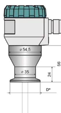
Tri- Clamp
