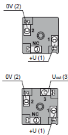
Connection diagram of the ULM level meter (variant -I) and inside view of the connector
