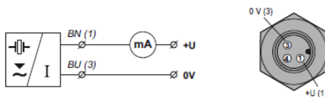
Connection diagram of the ULM level meter (variant -I) and inside view of the connector
